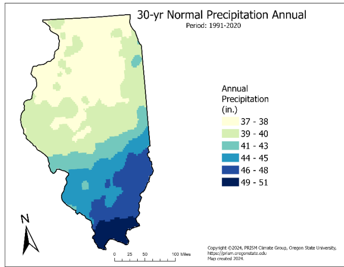
Figure 3. Normal mean precipitation (in.) from 1991–2020 in Illinois.
