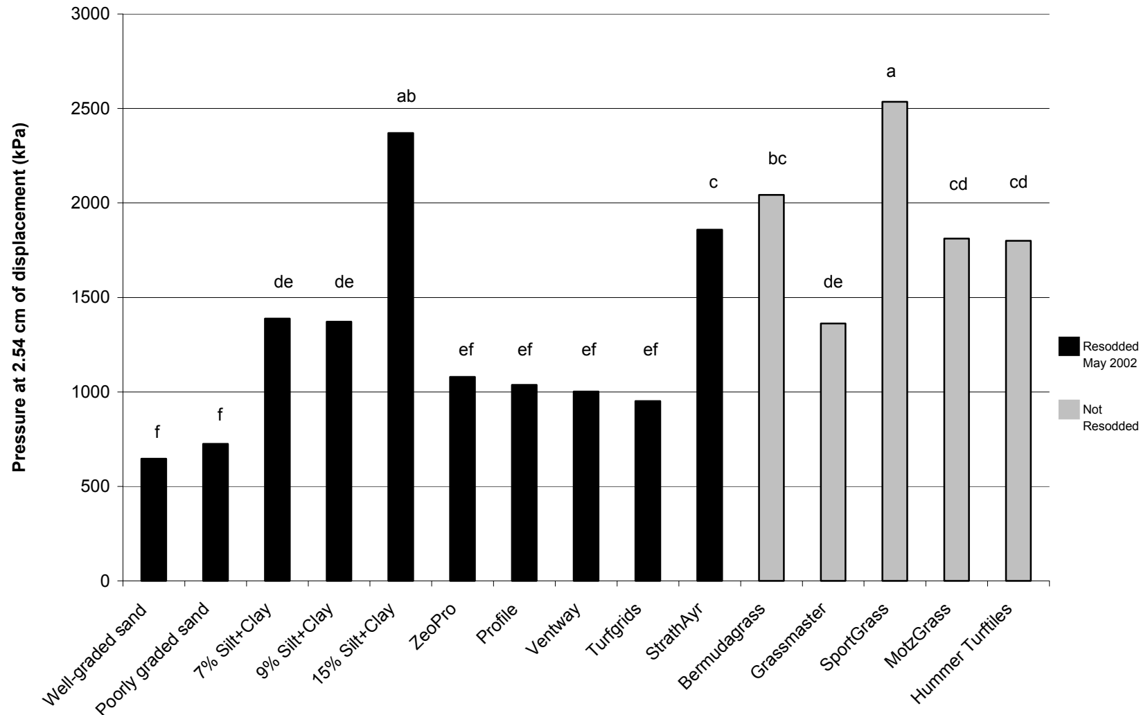
Figure 1. The effect of natural and artificial enhancements on the bearing capacity of the daily trafficked portion of treatments 26 Sept 2002.
