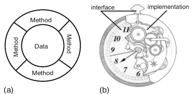
Figure 1. (a) An object in object-oriented programming with data and operations (methods) combined and (b) an interface and implementation of object-oriented programming (NeXT Software, Inc. 1992).
